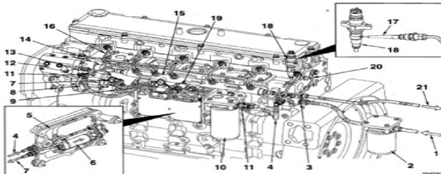
Cummins Common Rail Fuel System
