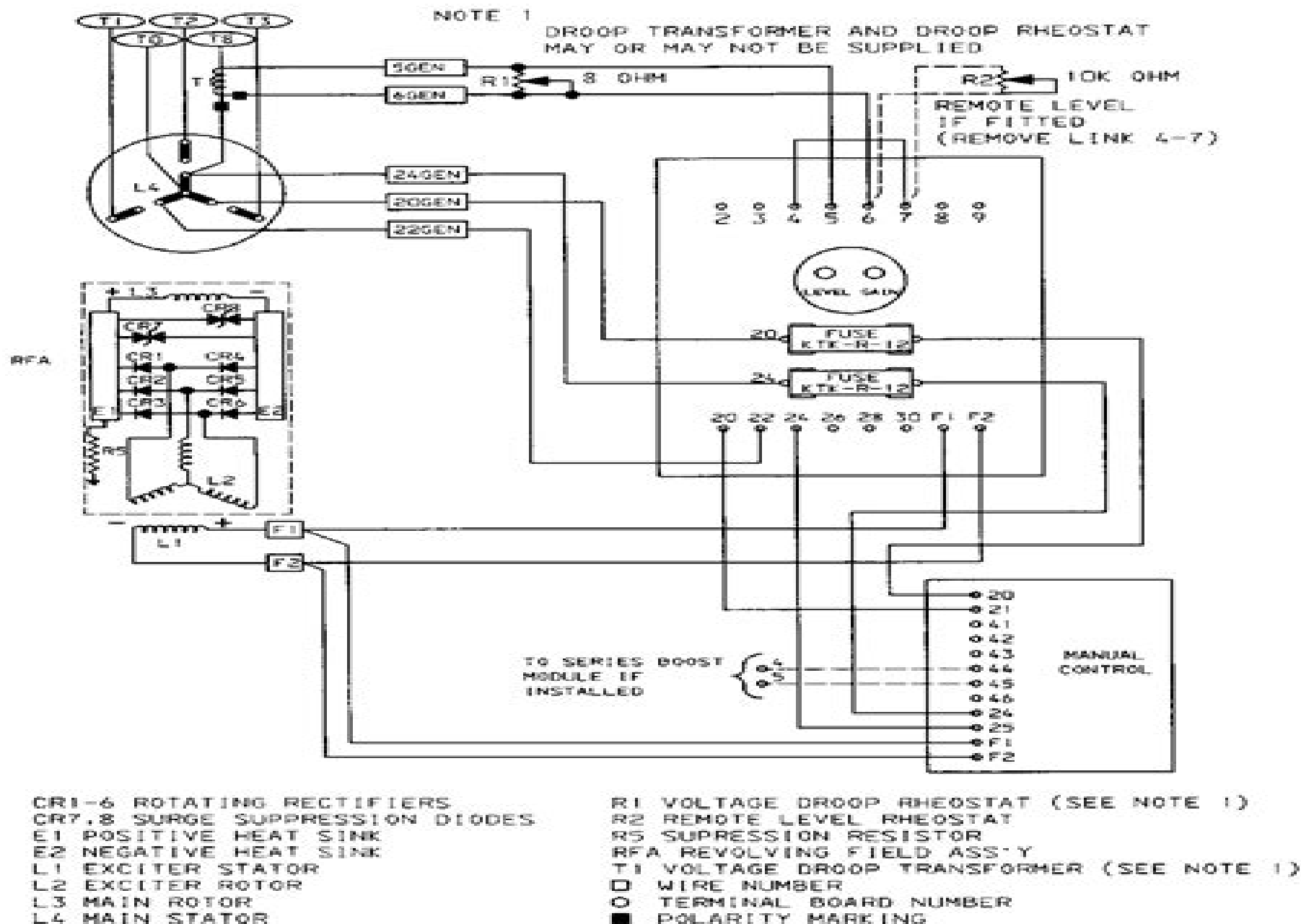
SR-4 GENERATOR SCHEMATIC (10/12 LEAD, SELF-EXCITED, 2 FUSE TYPE, & MANUAL CONTROL)
