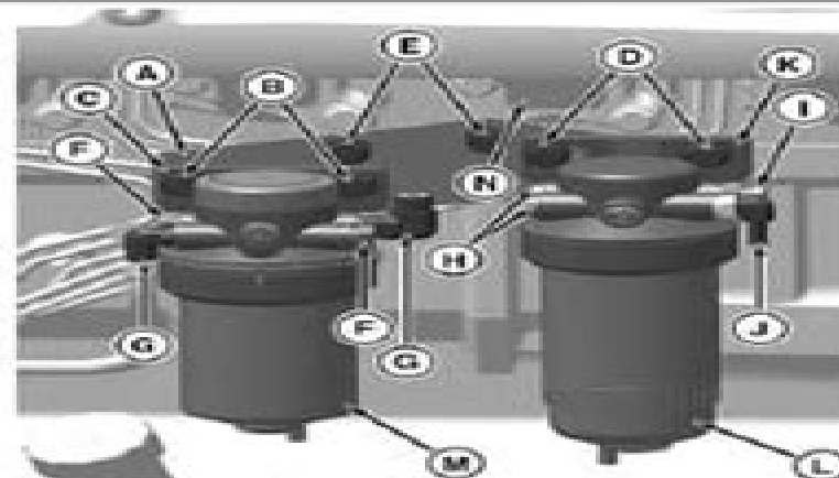
Primary and Secondary Fuel Filter Installation
