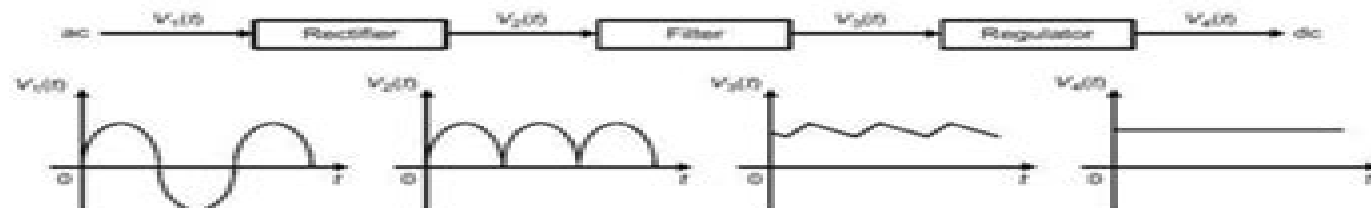
Figure 1: Convert AC to DC
