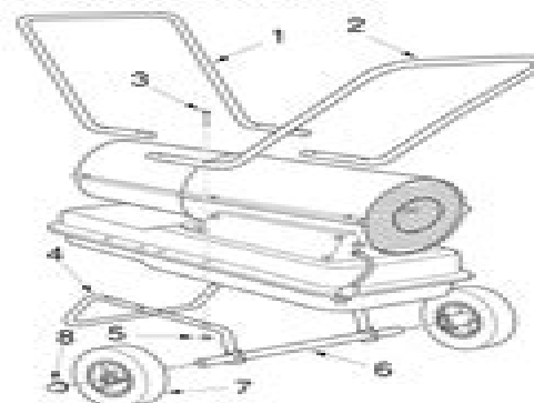
Figure 39 - Handle and Wheel Assembly
