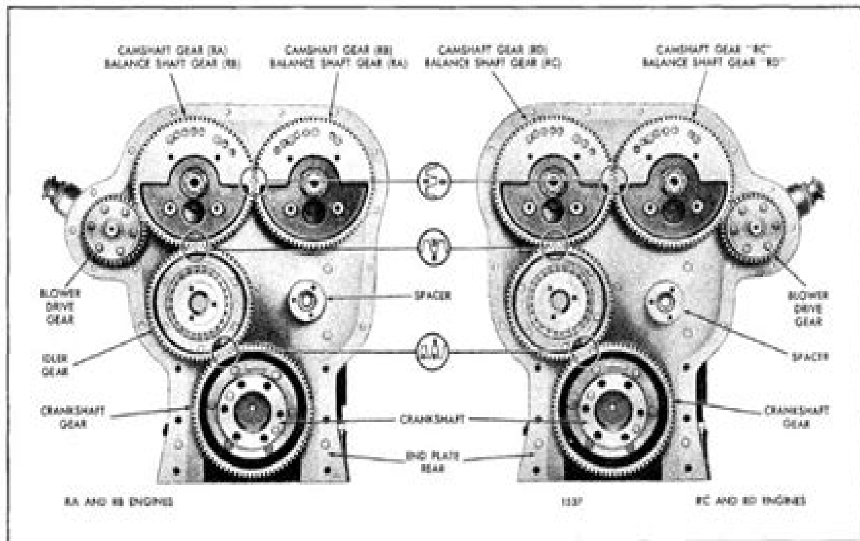
Fig. 2 - Gear Train and Timing Marks - Right Hand Rotation Engines (Standard Timing Shown)
