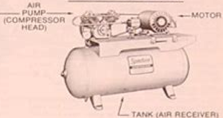
Figure 1 — Basic Air Compressor Nomenclature
