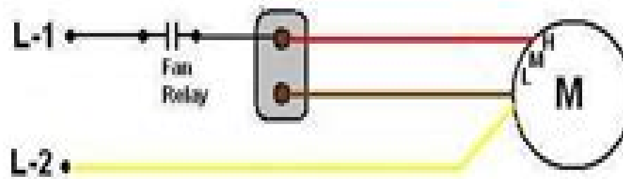
Original Single Speed Motor
