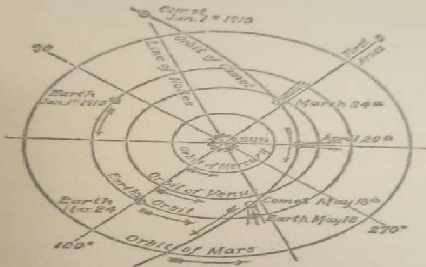
Relative Positions of Halley's Comet, the Earth, and the Sun.—1910.
