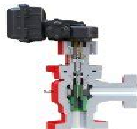
CAM30-DC multitrim choke valve (electric)
