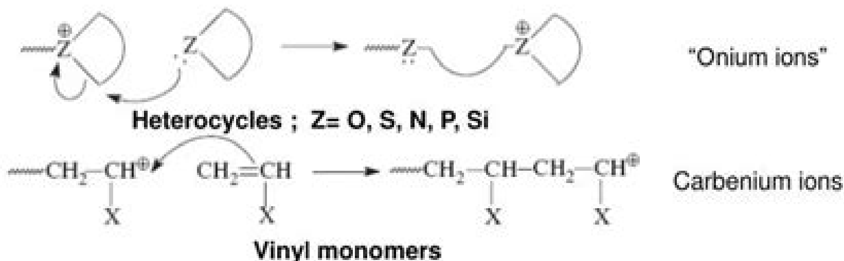
Scheme 1. Propagation reactions in cationic ring-opening and carbocationic polymerizations (counteranion omitted).
