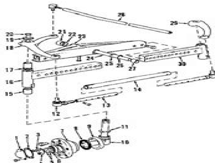
Fig. 2—Exploded view of Model 885N front axle, wheel spindle, hub and bearing assembly. Note shims (5) used to adjust bearings.
