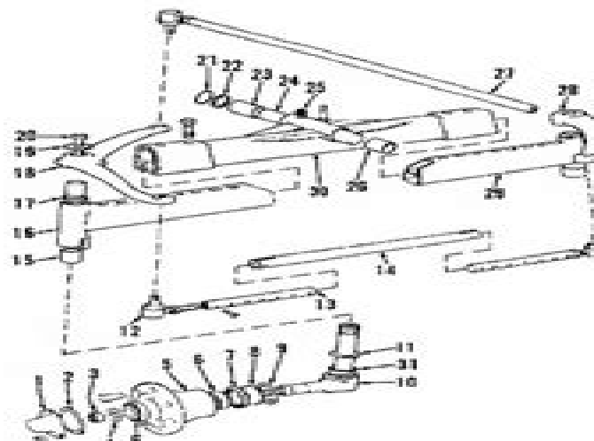
Fig. 1—Exploded view of front axle, wheel spindle, hub and bearing assembly typical of those used on Models 885 and 895. Model 885N is shown in Fig. 2. Oil seal is installed with lip away from inner bearing.
