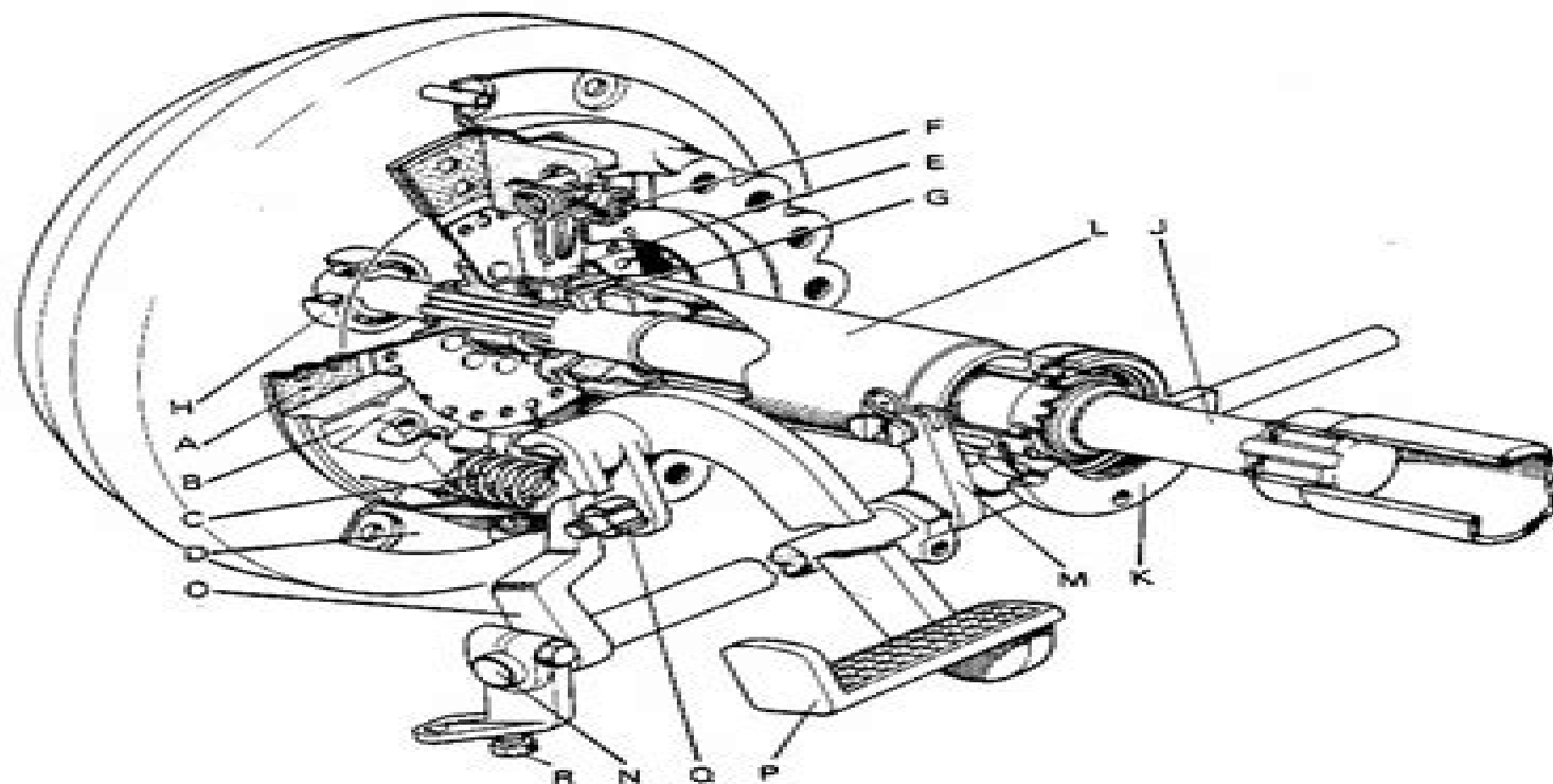
Figure 1 SINGLE PLATE CLUTCH — 990/880 TRACTORS
