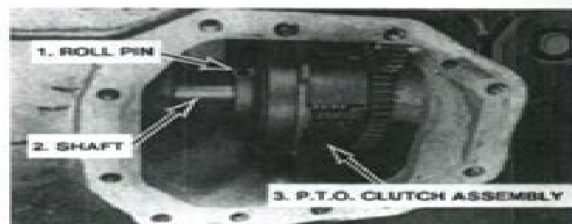
Fig. 88—Bottom view of pto clutch (cover removed).
