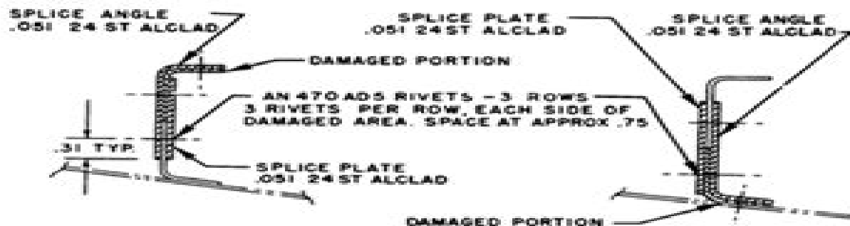
FIGURE 6-3. ENGINE MOUNT LOWER LONGERON REPAIR
