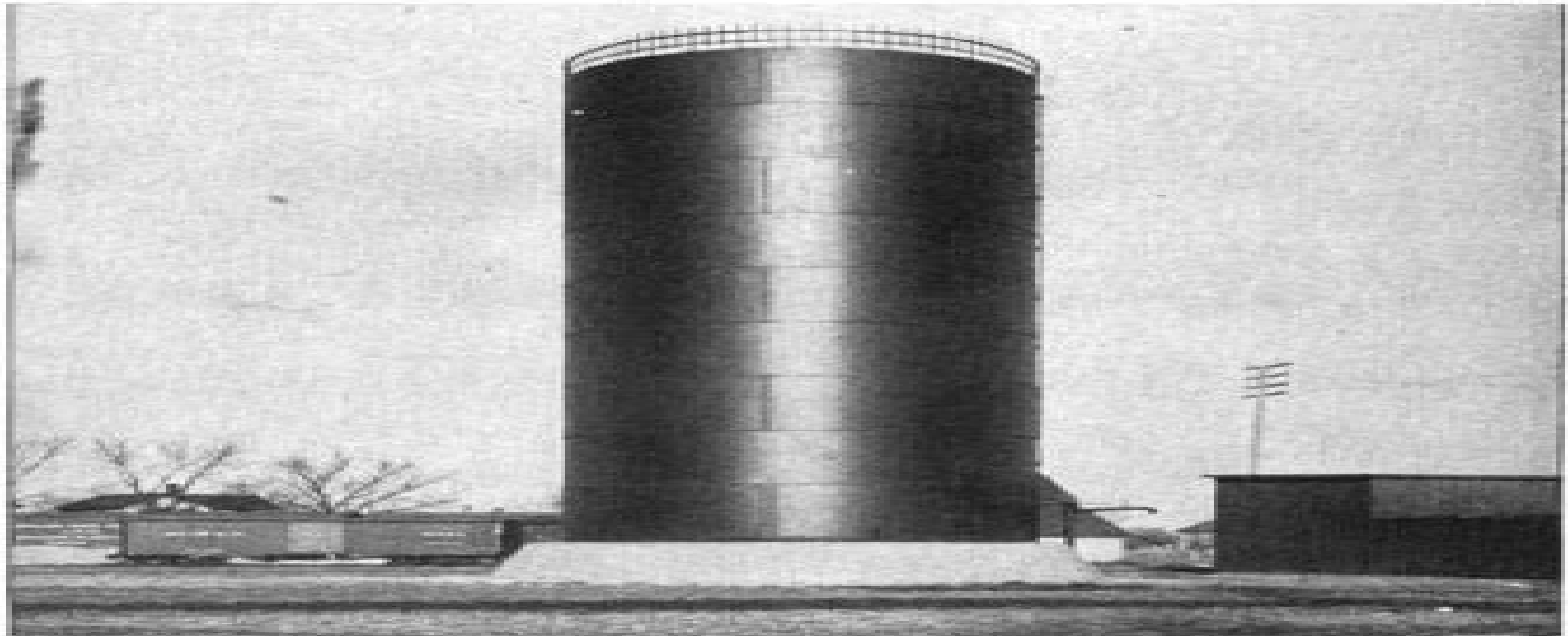
Steel Water Tank at Geneseo, Ill. C. R. I. and P. Ry. 25 feet Diameter, 60 feet high. Capacity, 220,000 gallons.
