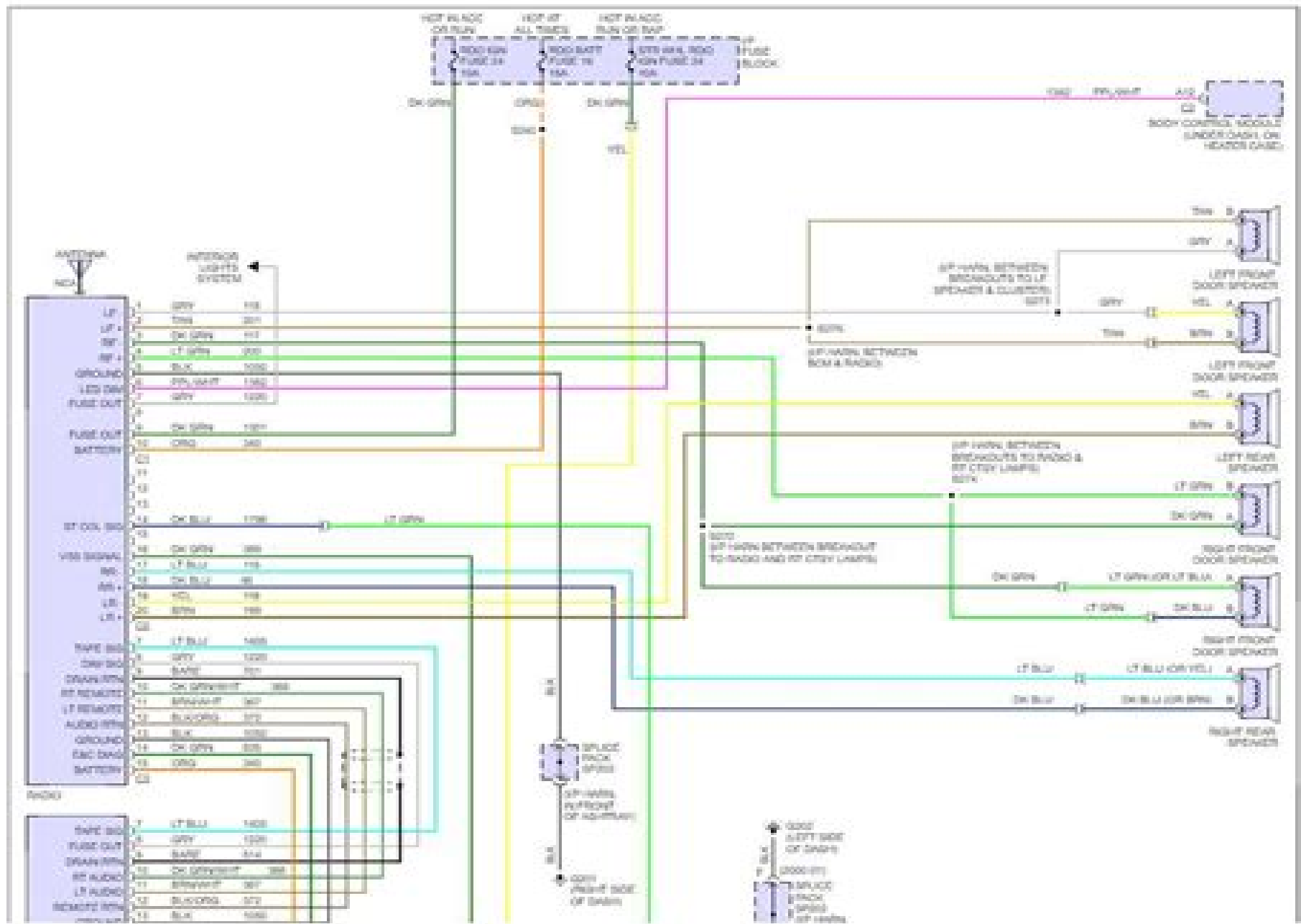
Fig 2. Radio Circuits, W/O Amplifier
