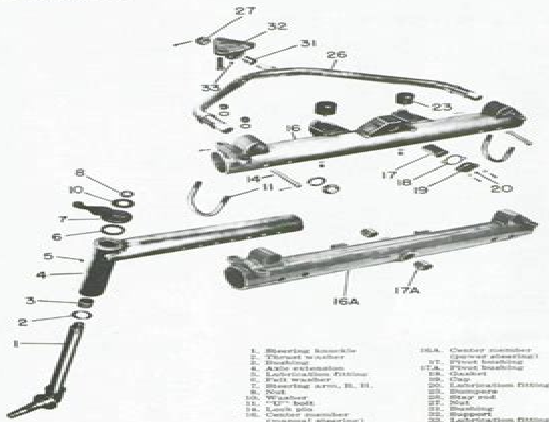
Fig. O1 — Exploded view of Rowcrop adjustable front axle assembly. Models equipped with manual steering use center (main) member (16); those equipped with power steering use center member (16A). Narrow froad power steering models use center member similar to (16A), but shorter than standard part.
