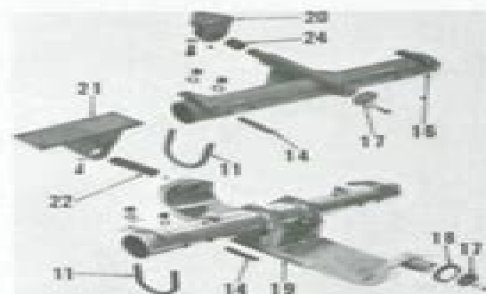
Fig. O2 — Axle center member used on short wheel base and utility model tractors.
