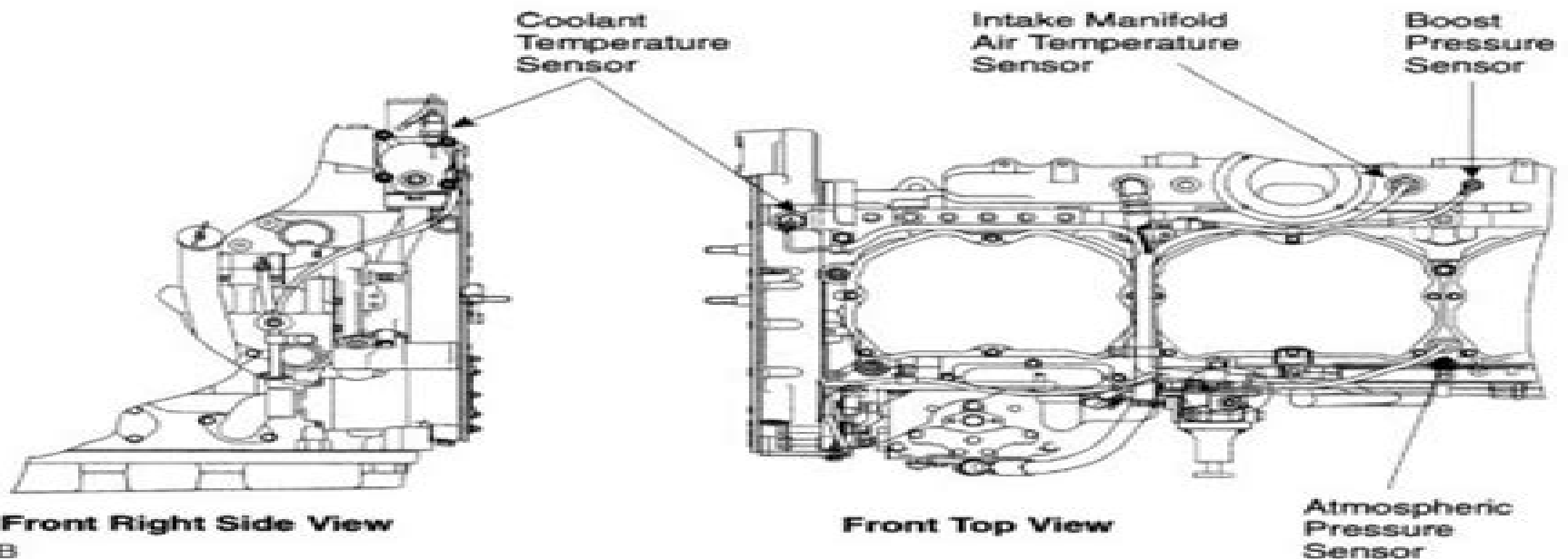
6-14 EMS component location, C-10 and C-12 Caterpillar engines. Left-side view (A) and right-side and top view (B). Courtesy Caterpillar Inc.
