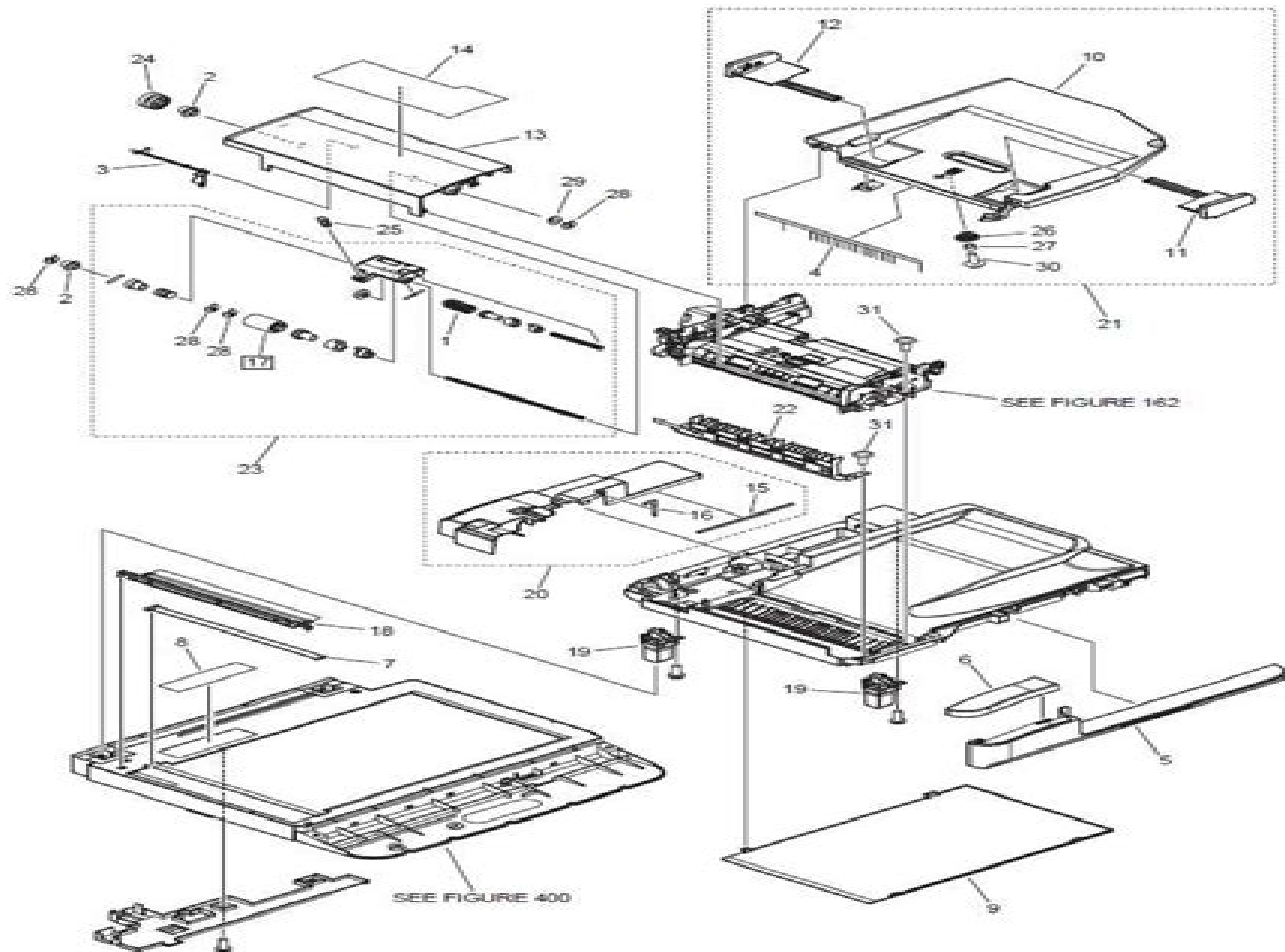
FIGURE 160 READER/ADF ASSEMBLY
