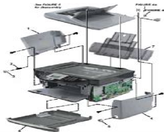
OUTER COVER, DOCUMENT FEED ASS'Y
