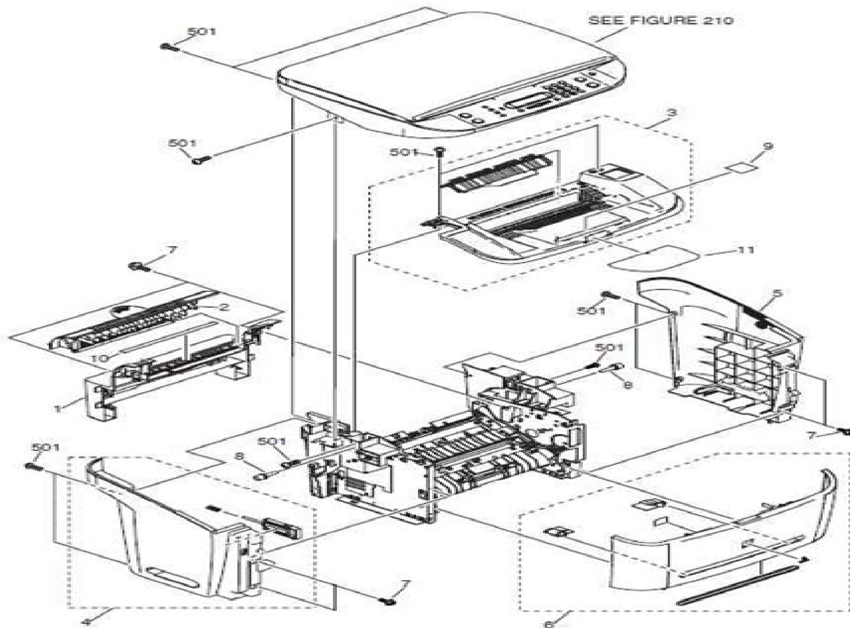
FIGURE 100 EXTERNAL COVERS, PANELS ,ETC.
