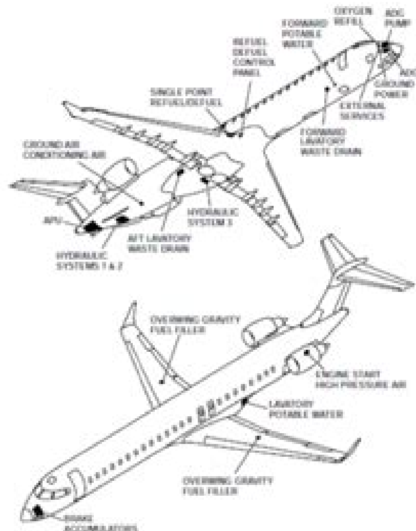
Airplane Service Points - 0000- Figure 01-20-4
