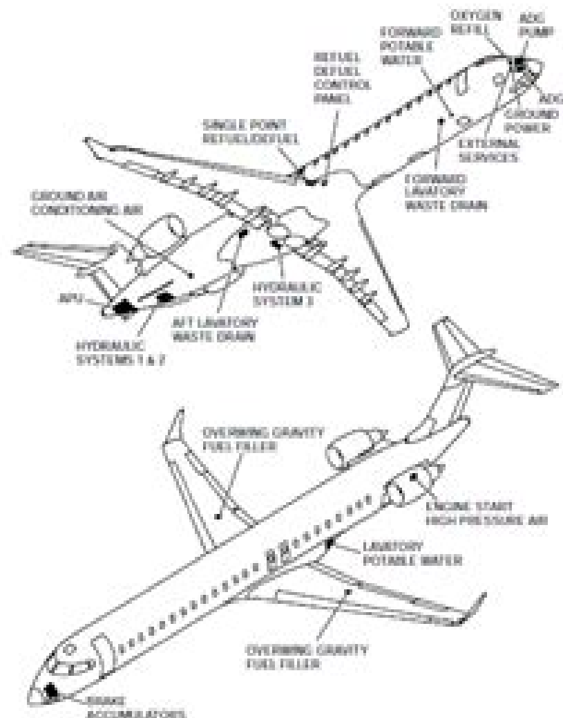
Airplane Service Points - (Continued) Figure 01-20-4
