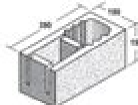
20.15 Corner Bond Beam
