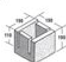
20.44 Knock-in Half Bond Beam
