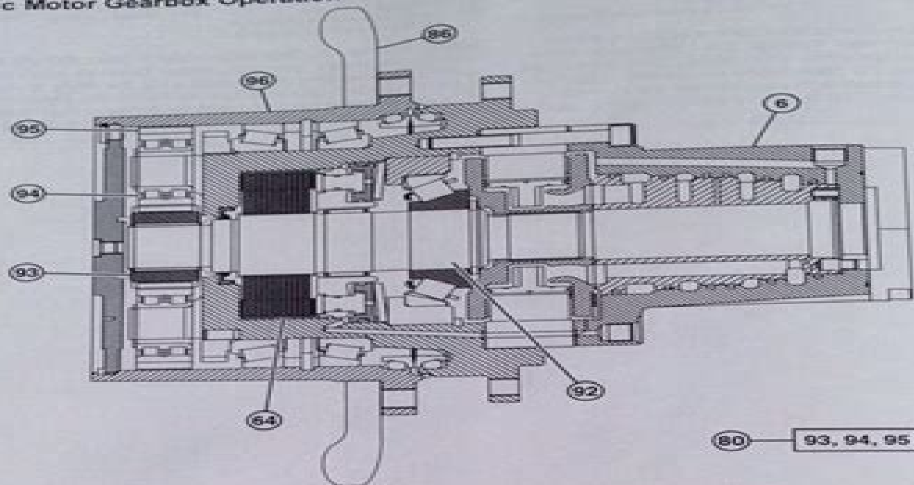
Hydrostatic Motor Gearbox Component Location (two speed motor shown)
