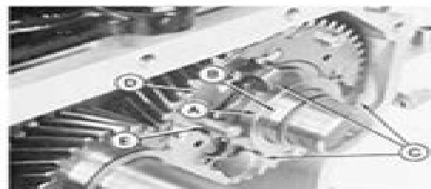
A—Governor Sleeve B—Camshaft C—Weights D—Weight Assembly Plate E—Locator Pin
