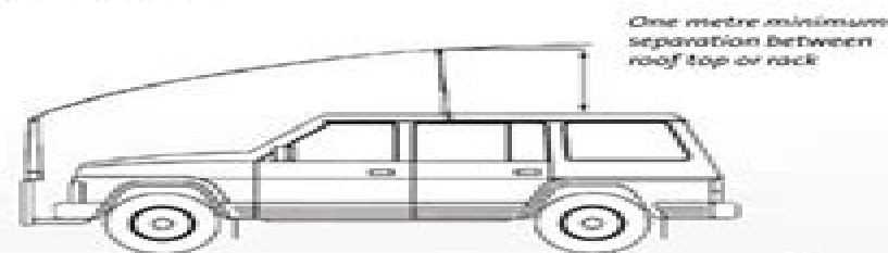
Antenna mounted on bull bar
