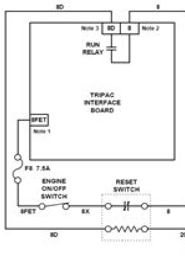
Partial Schematic Diagram - [Eng] Alarm Code
