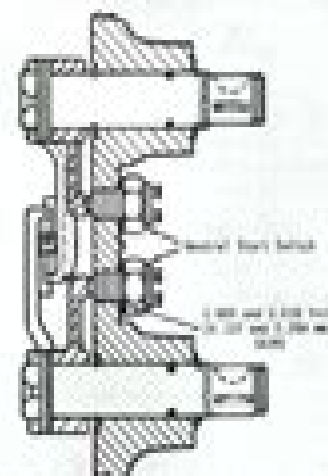
Fig. 98 - Cross-sectional view showing neutral start switch plate placement and shift shims. Note to text.
