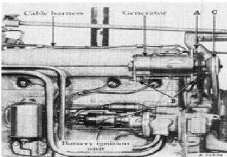
Illustr. 64 Generator, battery ignition unit and cable harness.
