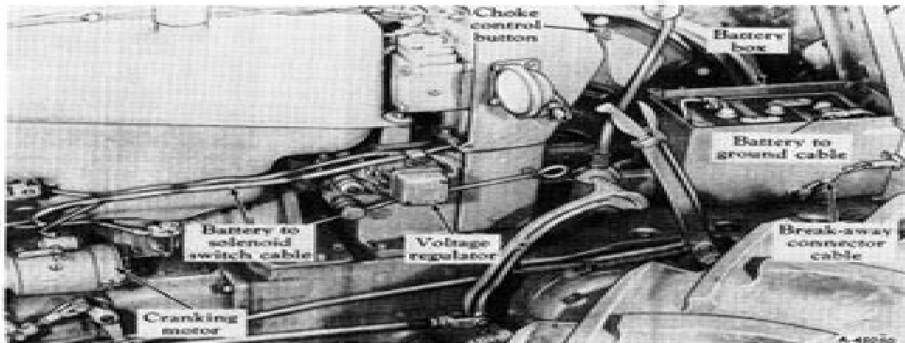
Illustr. 64A Cranking motor, battery box, and cables.
