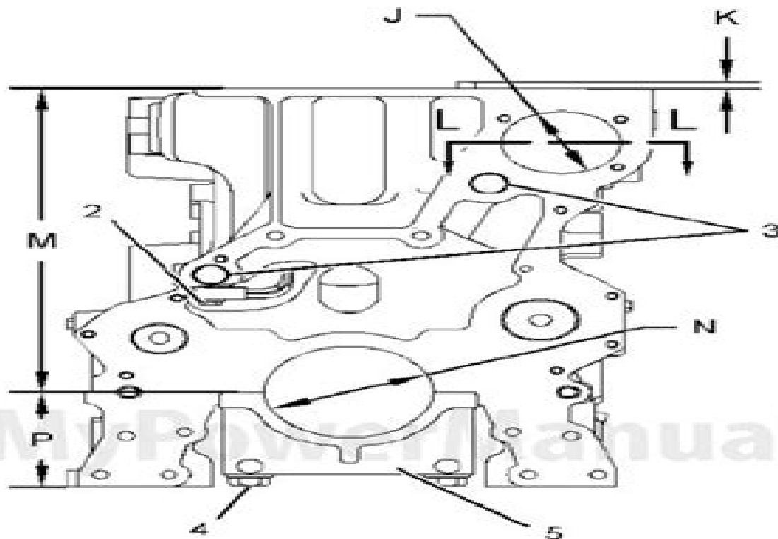
Illustration 3 Front face of the cylinder block
