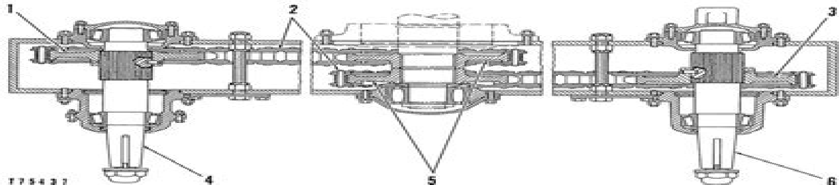
TANDEM DRIVE—RIGHT SIDE (Top View)
