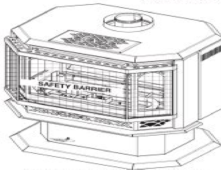
Model CS500-1 is made up of Model CDV5500-1 and Natural Vent Adapter Kit GS-150CT
