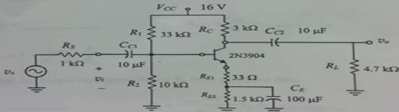
Figure 6: Common-emitter amplifier.
