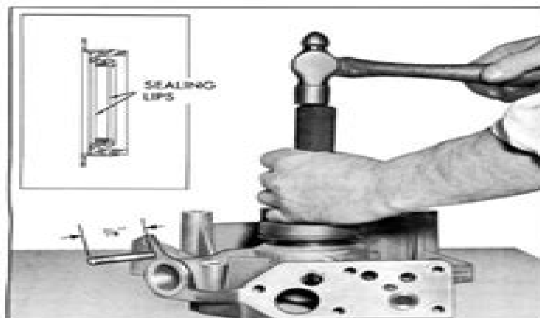
Fig. 114—Installing Rear Housing Seal
