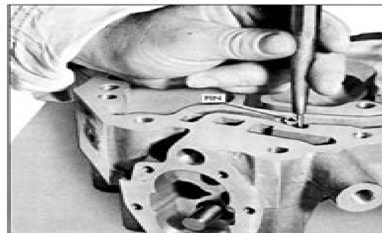
Fig. 116—Installing Pressure Regulator Groove Pin
