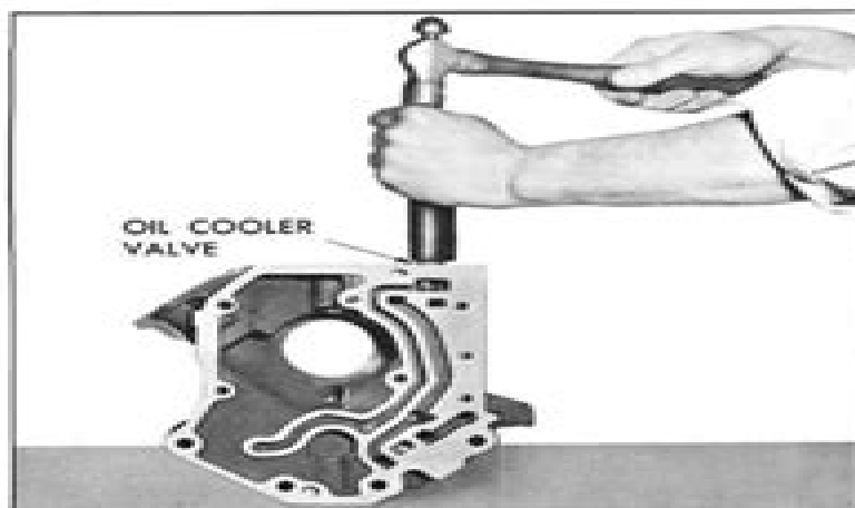
Fig. 115—Installing Oil Cooler By-Pass Valve
