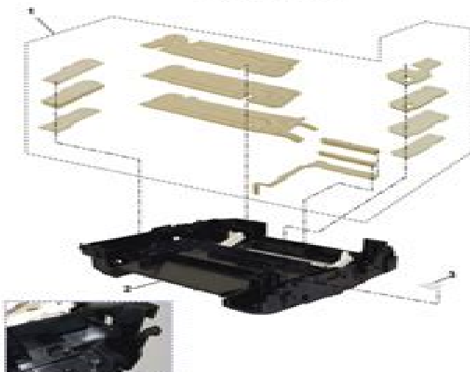
BOTTOM CASE UNIT & INK ABSORBER
