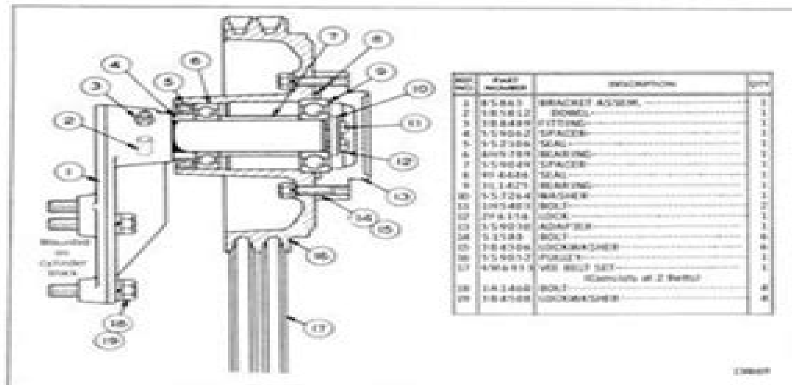
FAN DRIVE AND SUPPORT (751247 N/S) Serial No. 93J611 to 93J653 inclusive and 94J1363, 94J1556 to 94J1560 and 94J1562 to 94J1567 inclusive
