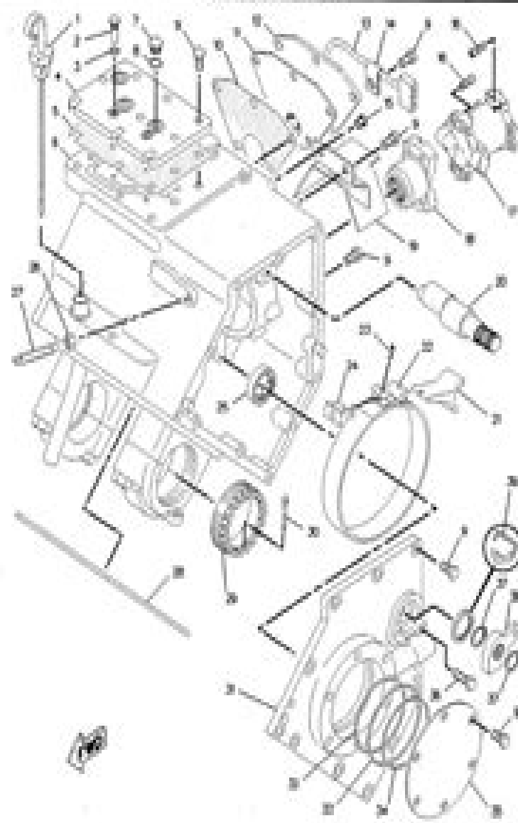
STEEL CASE & PARTS OF TRANSMISSION Type 2-57H 2NCT-67H, 4NCT-70H, 4NCT-81H, 5NCT-80H
