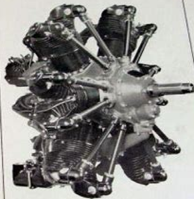
FIG. 2 THREE-QUARTER PROPELLER END VIEW
