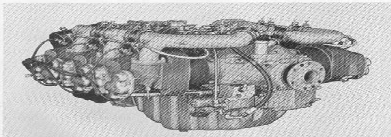
Figure 1-5. Three-Quarter Right Front View of the TSIO-360A and II.
