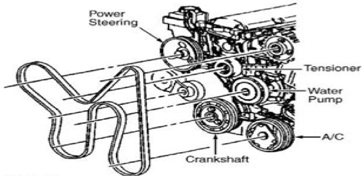
Fig. 7: Serpentine Belt Routing (2.2L "J" Body - With A/C) Courtesy of GENERAL MOTORS CORP.
