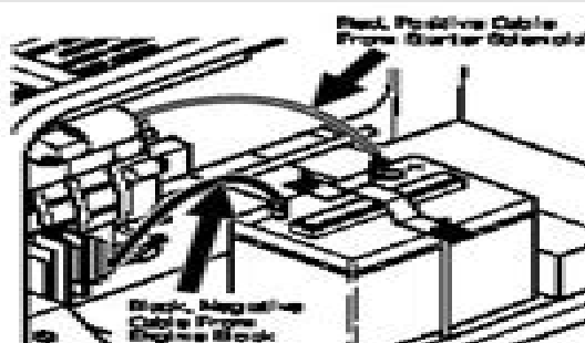
Figure 13 – Connecting Positive and Negative Cables to Battery
