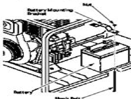
Figure 12 – Battery Hold-Down System
