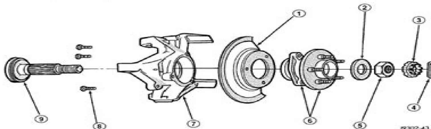
Fig. 3 Hub Bearing & Knuckle
