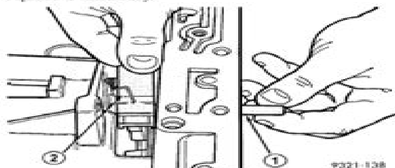
Fig. 76 Remove Guide Bracket Pivot Shaft
