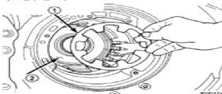
Fig. 74 Low/Reverse Piston Belleville Spring
