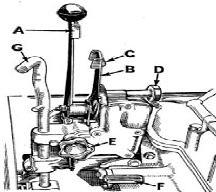
FIG. 1/5. Controls
