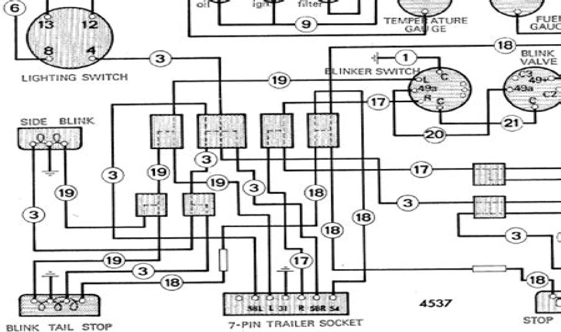
FIGURE 3/30. WIRING DIAGRAM
