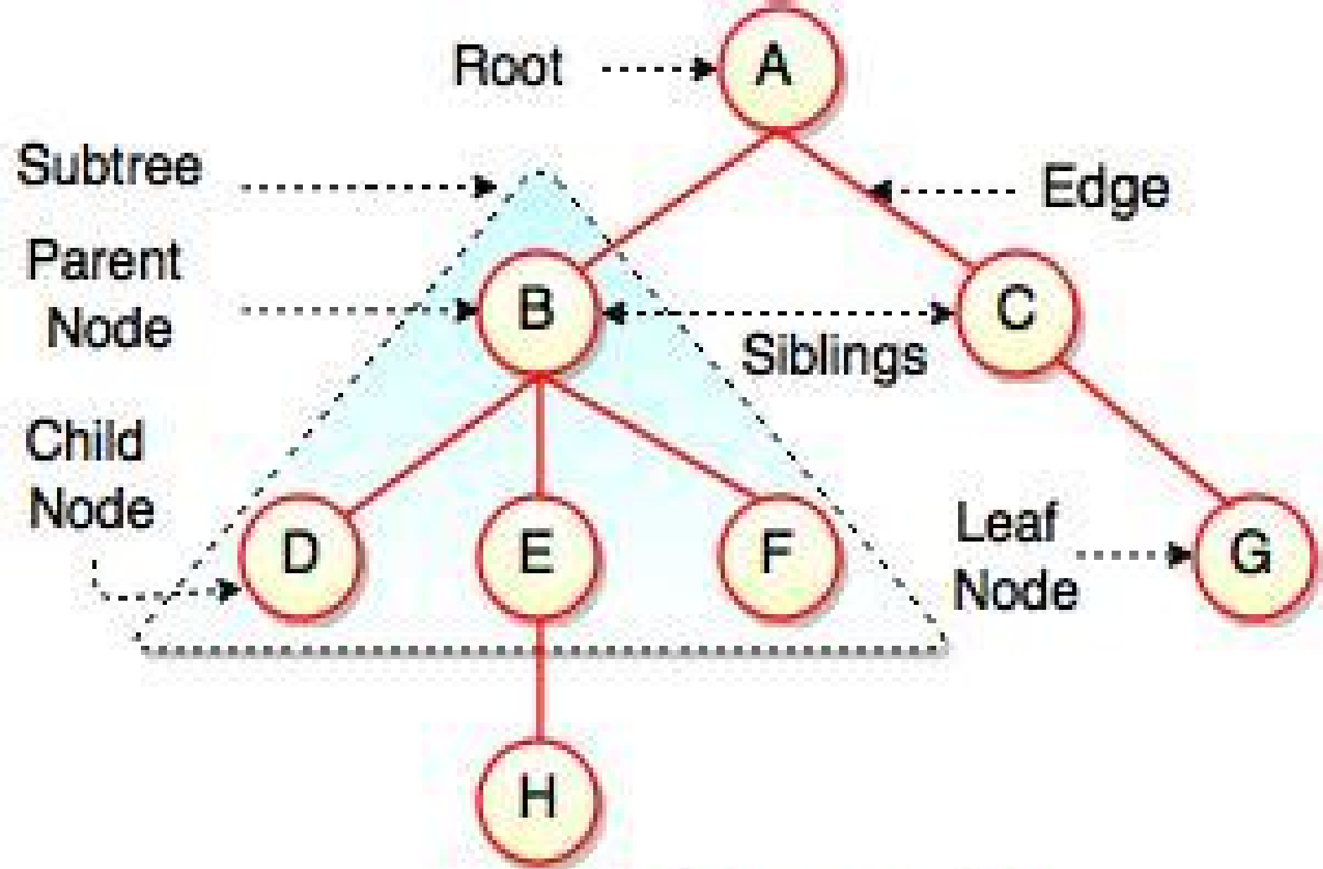
Fig. Structure of Tree
