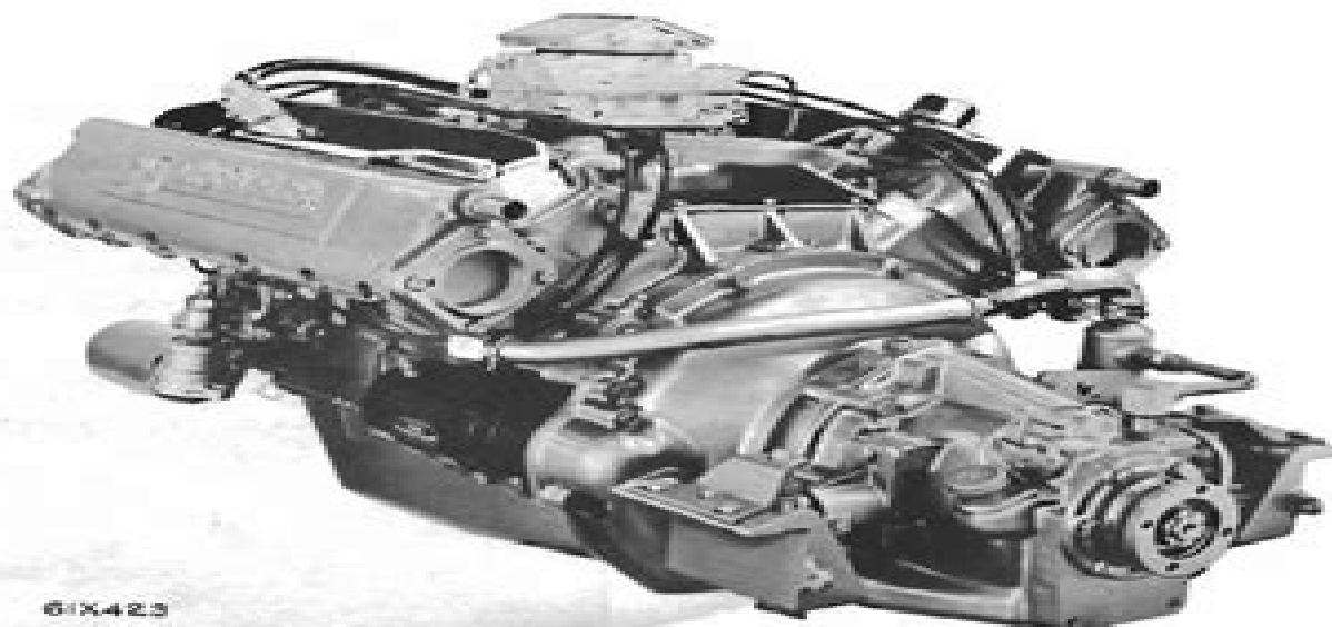
Fig. 3—Left Side View of Model M-413 Marine Engine
