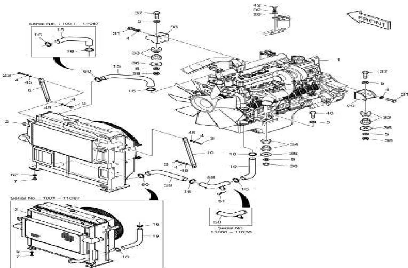
Fig. 1110 ENGINE MOUNTING
